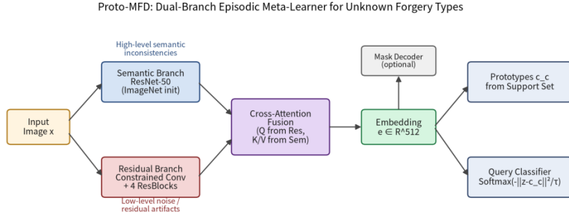
Figure 1. Architecture of Proto-MFD. The dual-branch encoder fuses semantic features from ResNet-50 with a learnable high-pass residual branch through cross-attention, producing a 512-d forensic embedding for nearest-prototype classification over the support set.
