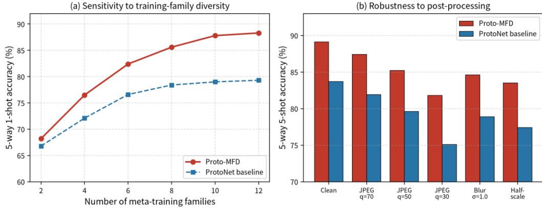
Figure 3. (a) Accuracy versus number of meta-training families; (b) robustness to post-processing degradations under 5-way 5-shot.
