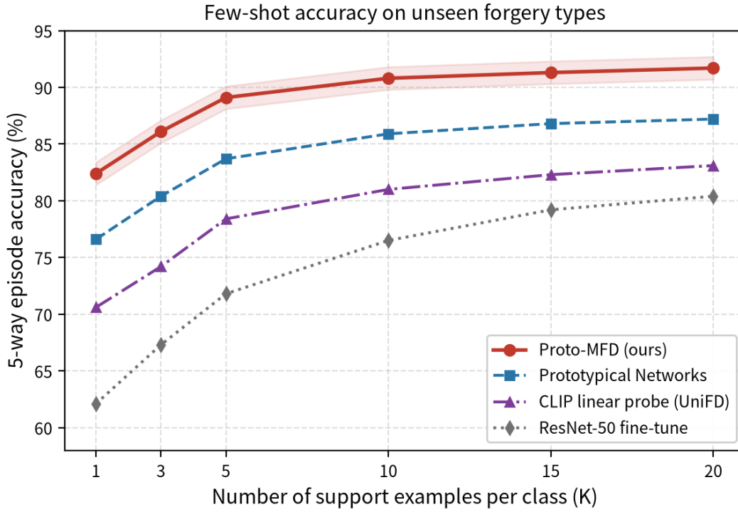
Figure 2. Accuracy versus number of support examples per class (K). Proto-MFD (red solid) compared with prototypical networks, CLIP linear probe, and plain ResNet-50 fine-tuning. Shaded band denotes 95% bootstrap CI.
